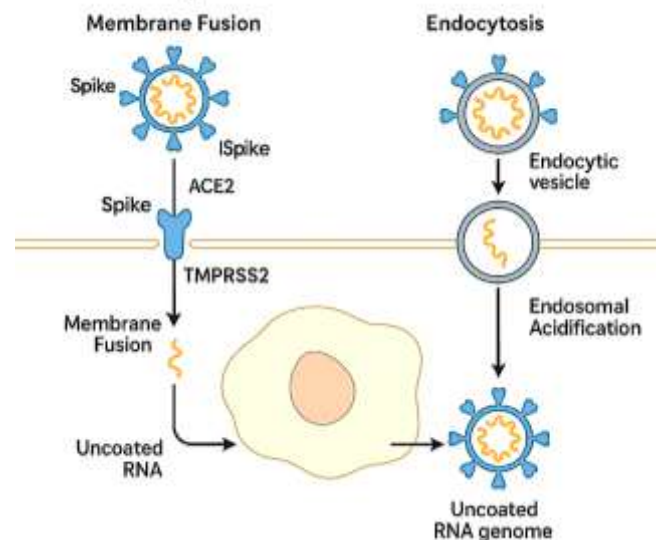
Figure 1: Schematic of Viral Entry Mechanisms Viral Entry Mechanisms of SARS-CoV-2
