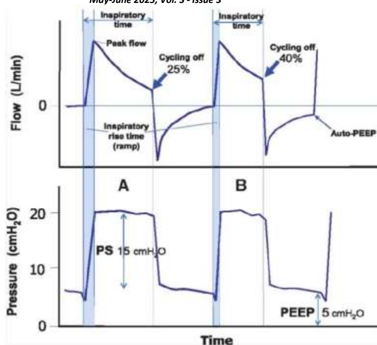
Pressure and flow curves in non-invasive pressure support ventilation (NIPSV). (A) Non-invasive pressure support ventilation delivered with a cycling off of 25% of the maximal peak flow. (B) Decrease of the inspiratory time after the reduction of the ramp and the increase of the cycling off to 40%. Example of flow curve with Auto-PEEP (the expiratory flow does not arrive to 0). PEEP, positive end expiratory pressure; PS, pressure support.
